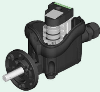
With set of cams. Yankee and flange
